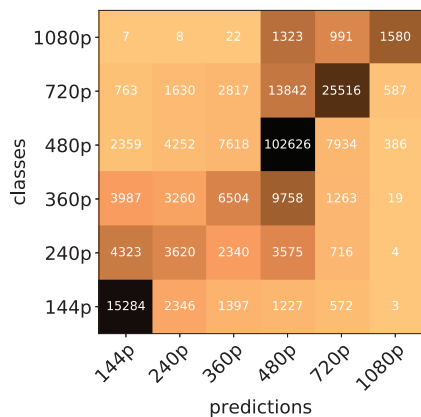
Fig. 1. Confusion matrix for kNN-based video resolution prediction.
